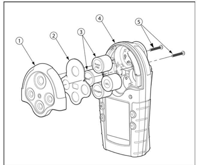
Figure 15. Replacing a Sensor or Sensor Filter
