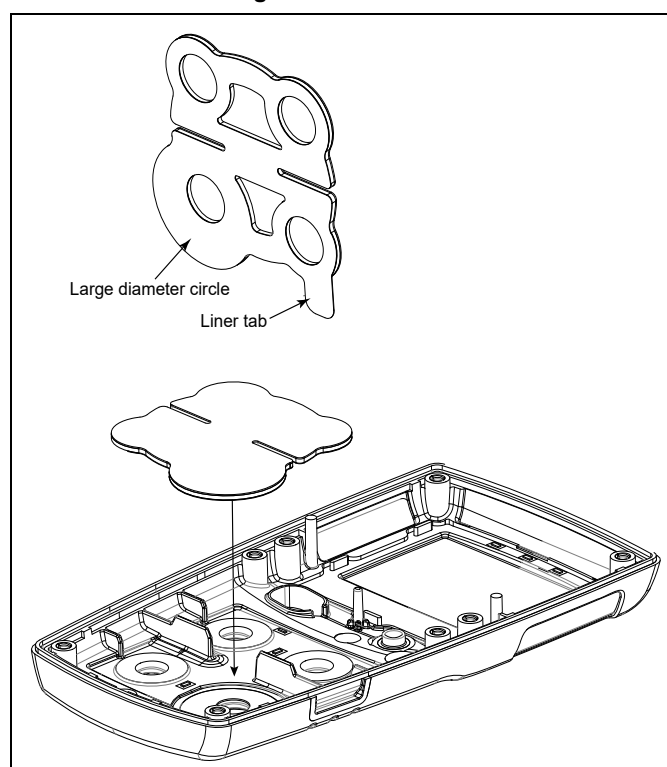
Figure 10. Liner Tab
