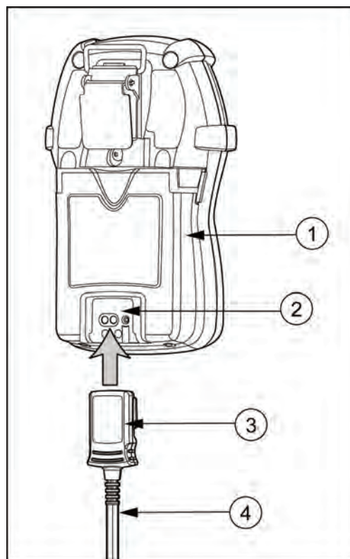
Figure 2. Connecting the IR Link
